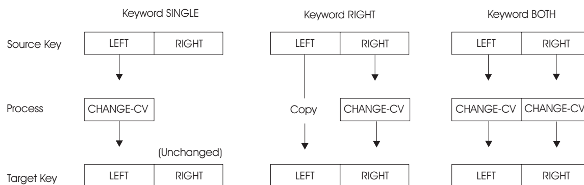
Figure 19. Control Vector Translate Callable Service. In this figure, CHANGE-CV means the requested control vector translation change; LEFT and RIGHT mean the left and right halves of a key and its control vector.
