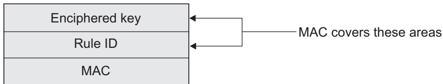
Figure 2. Simplified RKX key-token structure
