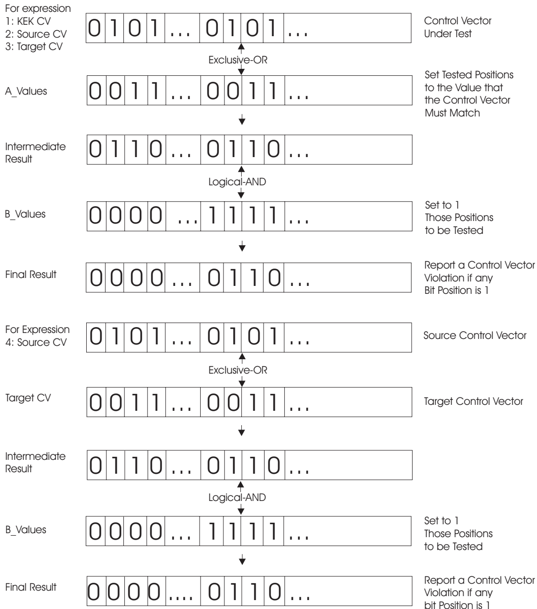
Figure 18. Control Vector Translate Callable Service Mask_Array Processing
