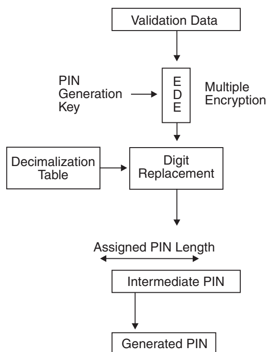
Figure 20. 3624 PIN Generation Algorithm
