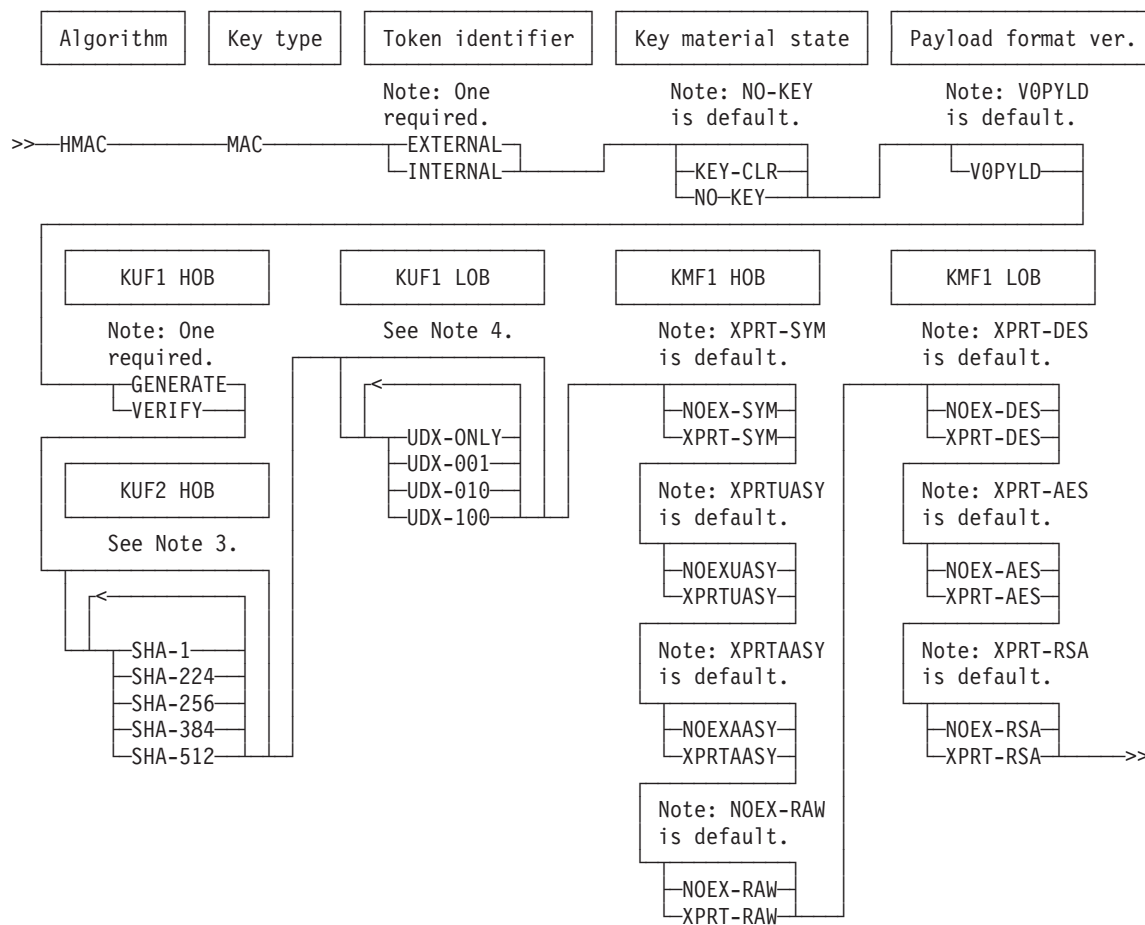
Figure 10. Key_Token_Build2 keyword combinations for HMAC MAC keys
