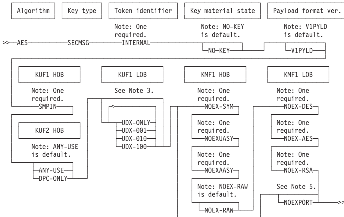
Figure 17. Key Token Build2 keyword combinations for AES SECMSG keys
